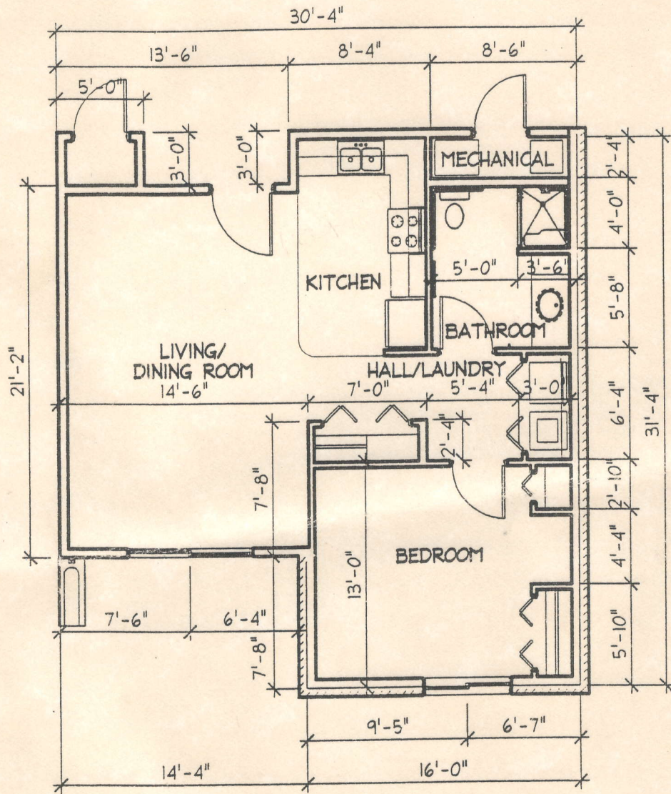
ONE BEDROOM APARTMENT 713 sq. ft.
